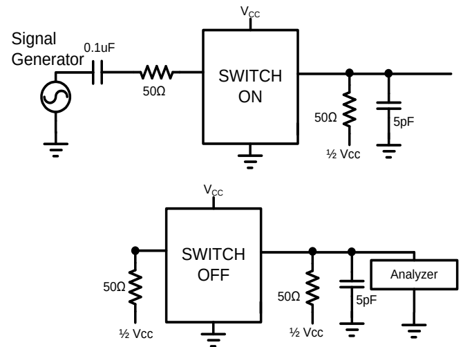
Figure 9 Crosstalk
