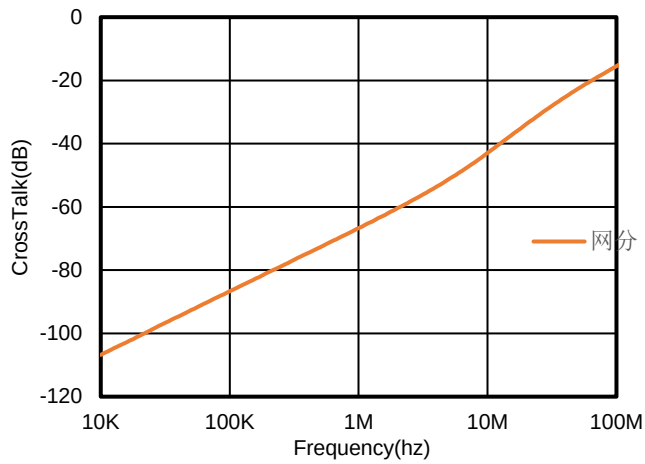
Figure 1. Off-Isolation, V_{CC} = 5V , V_{EE} = -8V
