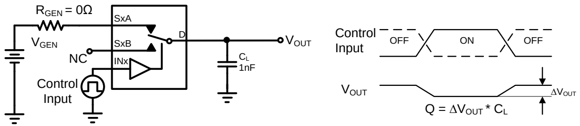
Figure 7 Charge Injection
