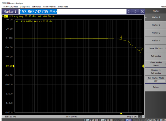
Figure 3. Bandwidth, V_{CC} = 5V , V_{EE} = -8V
