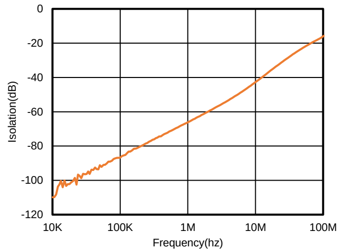
Figure 2. Crosstalk, V_{CC} = 5V , V_{EE} = -8V
