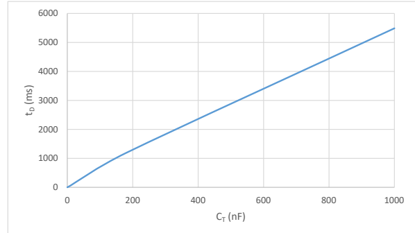
Figure 2. Reset Delay Time vs C_T
