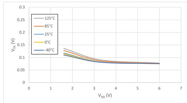
Figure 4. Low-level Reset Voltage vs Supply Voltage
