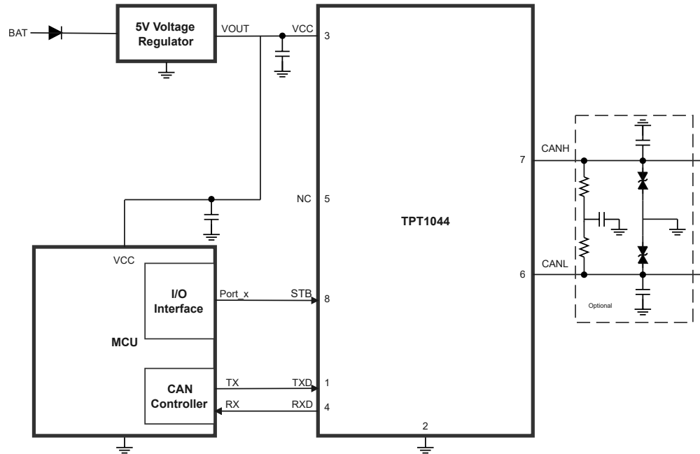
Figure 7. TPT1044 Typical Application Circuit
