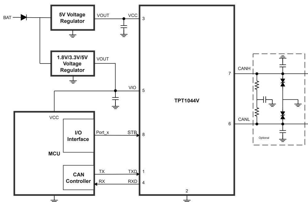
Figure 6. TPT1044V Typical Application Circuit
