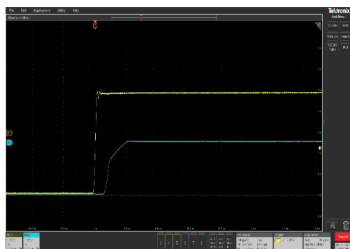
Figure 9. Step Response, V_{IN} = 5\text{ V} , C_{IN} = 1\text{ }\mu\text{F} , C_{OUT} = 1\text{ }\mu\text{F} , 200\text{ }\mu\text{s/div}
