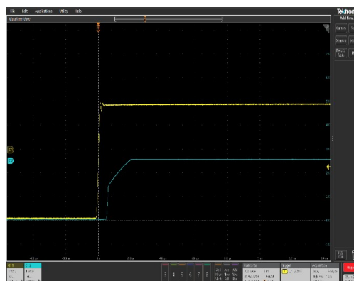
Figure 8. Step Response, V_{IN} = 5\text{ V} , C_{IN} = 1\text{ }\mu\text{F} , C_{OUT} = 0.1\text{ }\mu\text{F} , 200\text{ }\mu\text{s/div}
