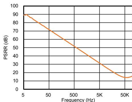
Figure 7. PSRR vs. Frequency
