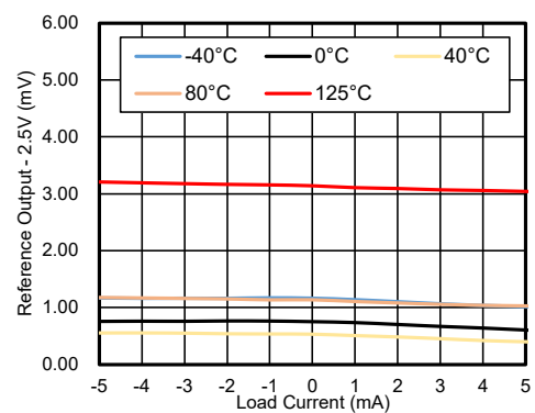
Figure 6. Output Voltage vs. Load Current
