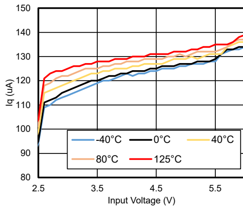
Figure 3. I_Q vs. Input Voltage
