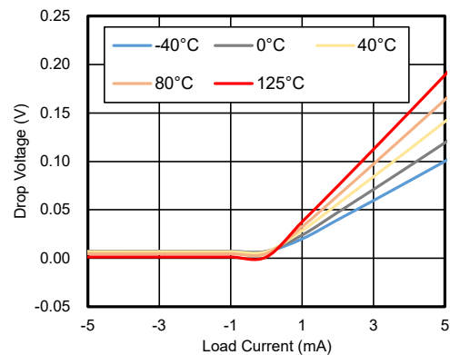
Figure 4. Drop Voltage vs. Load Current
