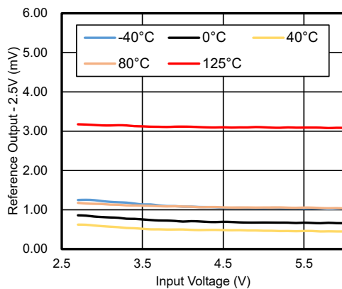
Figure 5. Output Voltage vs. Input Voltage
