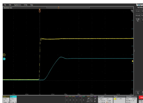
Figure 10. Step Response, V_{IN} = 5\text{ V} , V_{IN} = 5\text{ V} , C_{IN} = 1\text{ }\mu\text{F} , C_{OUT} = 10\text{ }\mu\text{F} , 200\text{ }\mu\text{s/div}
