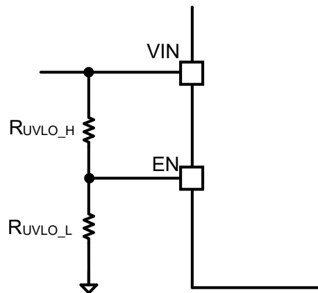
Figure 8. UVLO Adjustment
