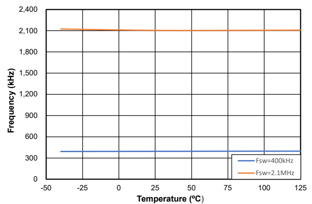
Figure 4. Switching Frequency
