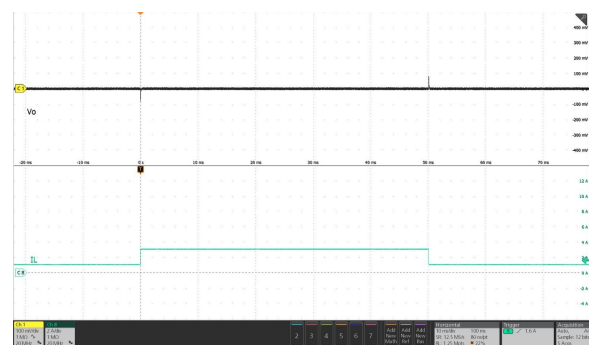
Figure 23. Load Transient
