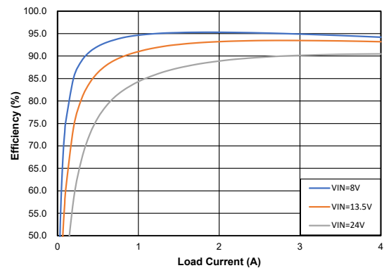
Figure 15. Efficiency
