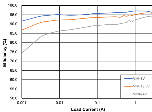
Figure 12. Efficiency
