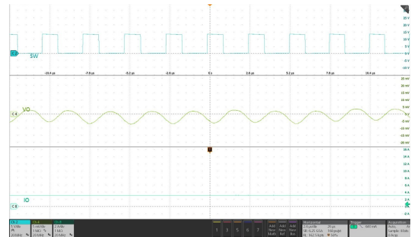
Figure 21. Switching Waveform and Output Ripple
