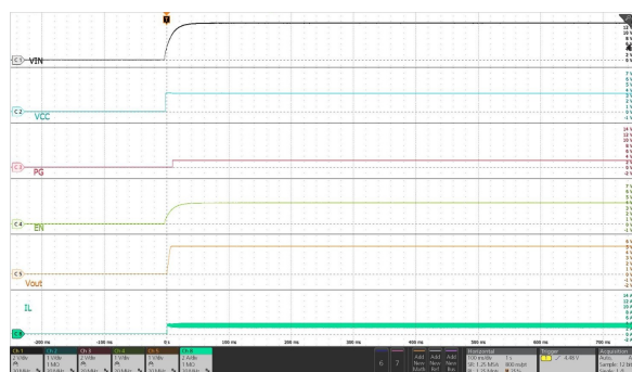
Figure 28. Power up by Inputs
