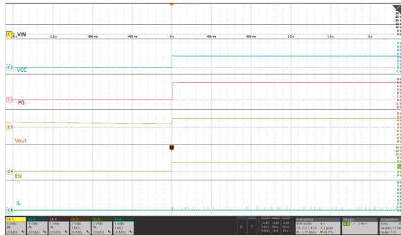
Figure 32. Power up by Enable
