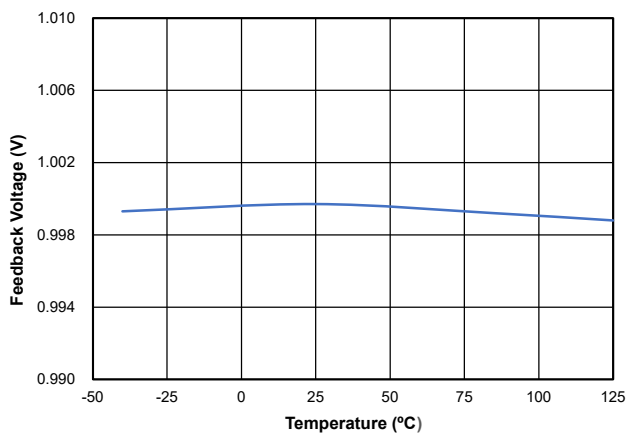
Figure 3. Feedback Voltage
