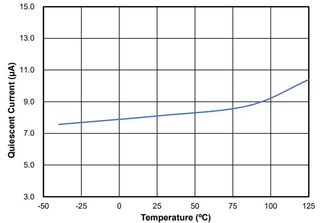
Figure 2. Quiescent Current
