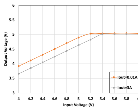
Figure 10. Low Drop-out Voltage
