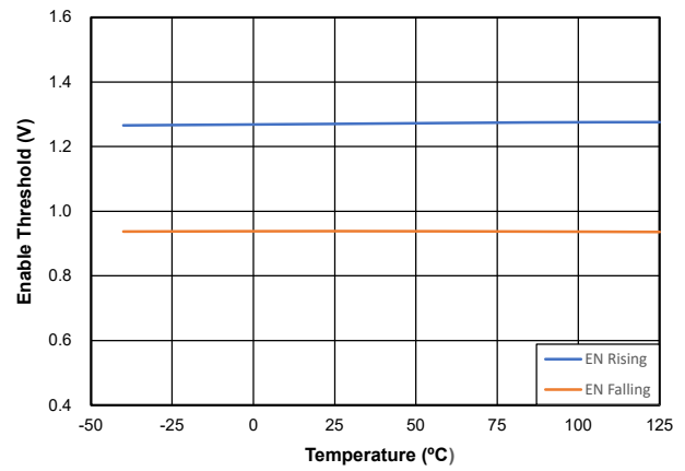
Figure 6. Enable Thresholds
