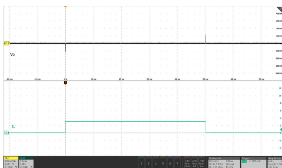
Figure 22. Load Transient
