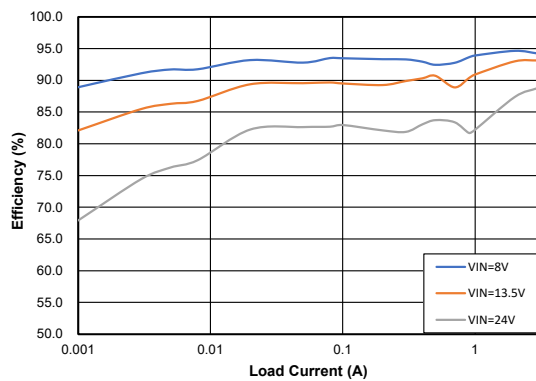
Figure 14. Efficiency
