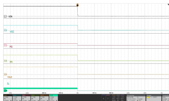
Figure 29. Power down by Inputs
