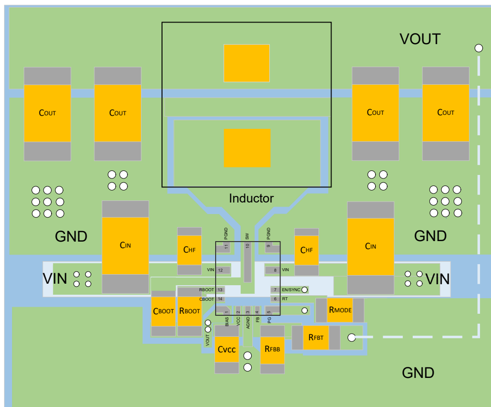
Figure 44. Layout Example
