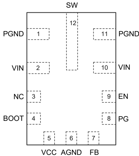
TPP36207Q QFN2X3-12 Top View
