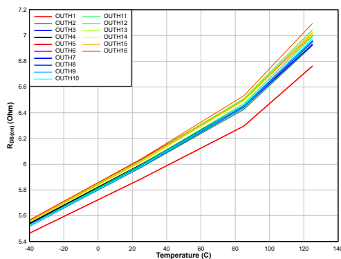
Figure 5. High-side On-Resistance
