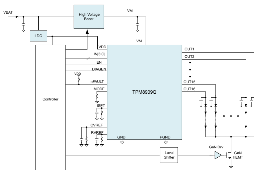
Figure 14. TPM8909/TPM8909Q Application Diagram
