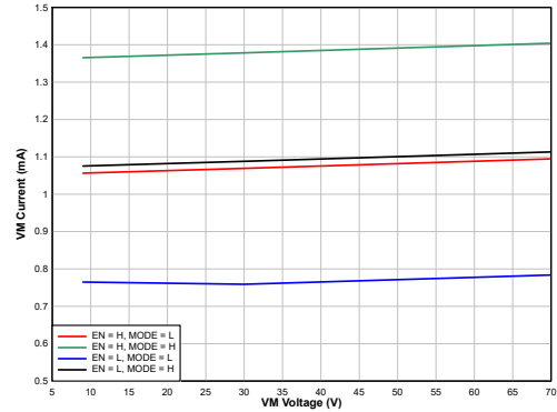
Figure 2. VM Current vs. VM Voltage
