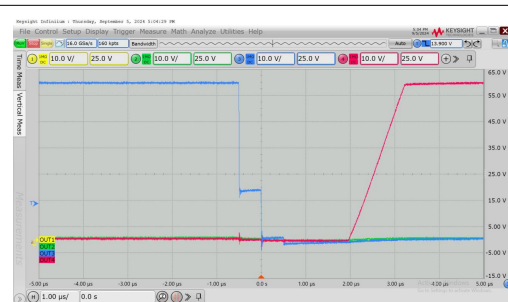
Figure 16. Discharge After Charging
