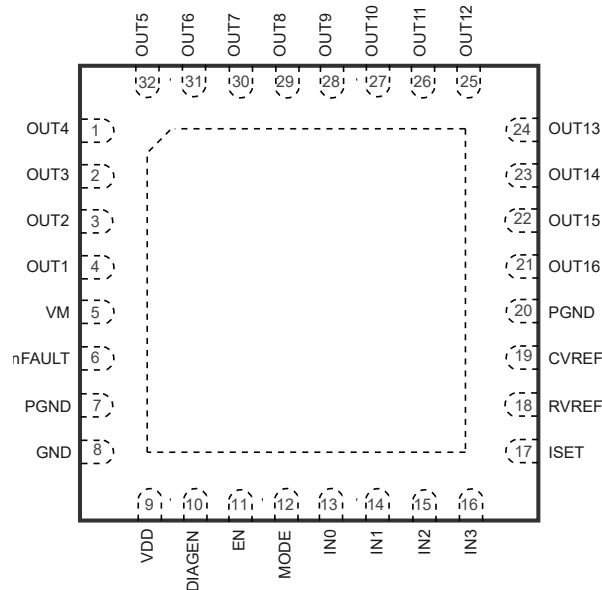
TPM8909/TPM8909Q QFN5X5-32 Package Top View
