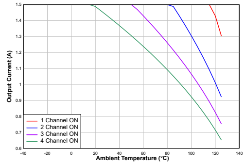
Figure 16. Output Current Capability - Parallel Mode
