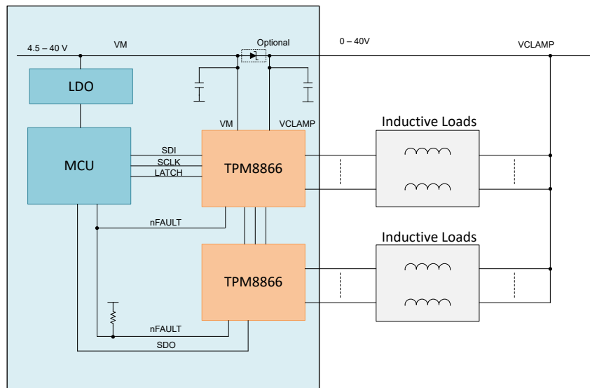
Figure 20. Typical Application Circuit
