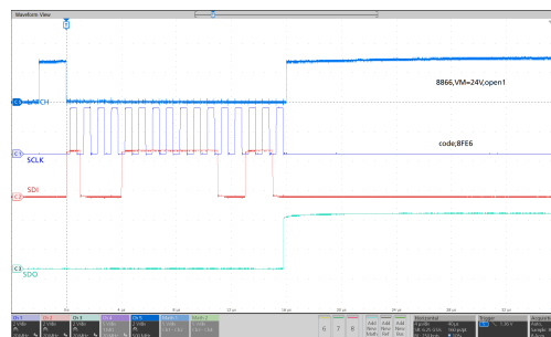
Figure 18. Serial Communication Write
