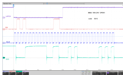
Figure 19. Serial Communication Read
