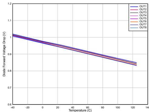
Figure 5. Forward Diode Drop vs. Temperature
