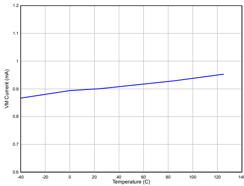
Figure 3. Quiescent Current vs. Temperature
