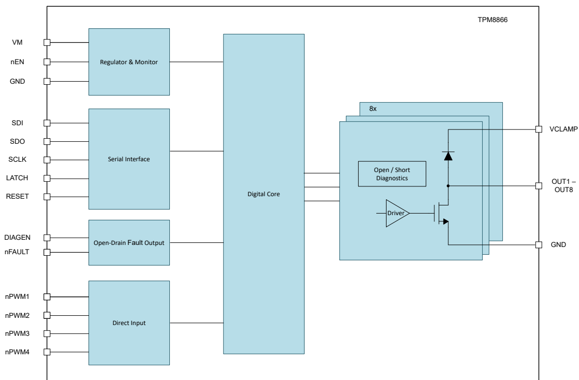
Figure 17. Functional Block Diagram
