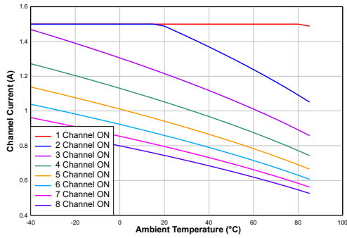
Figure 15. Output Current Capability
