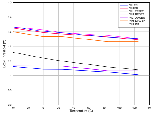
Figure 1. Logic Input Threshold vs. Temperature
