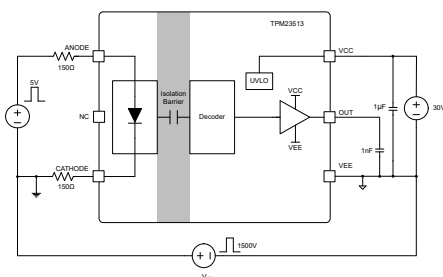
Figure 3. CMTI Test Circuit
