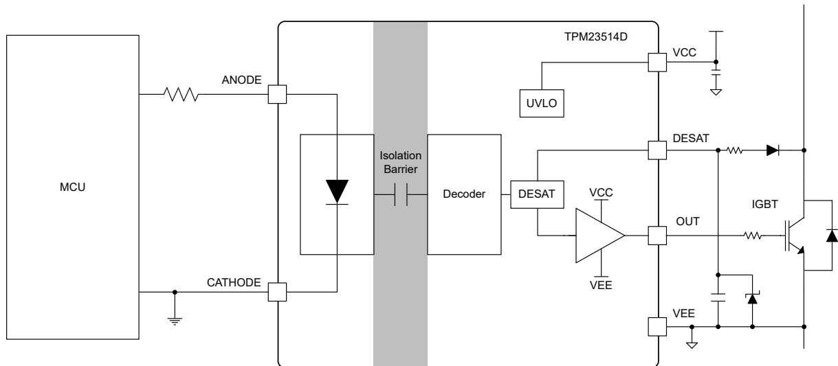
Figure 20. TPM27514D Desaturation Protection Application Diagram
