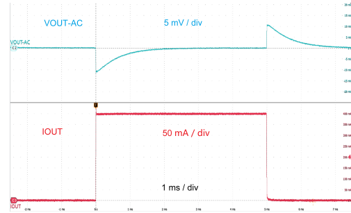
Figure 8. Load Transient
