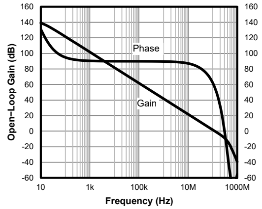
Figure 14. Open-Loop Gain and Phase
