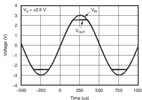
Figure 16. No Phase Reversal
