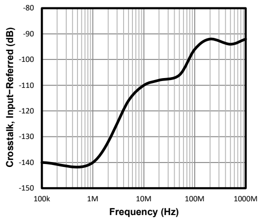
Figure 10. Channel-to-Channel Crosstalk
