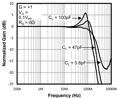
Figure 3. Frequency Response for Various C_L
