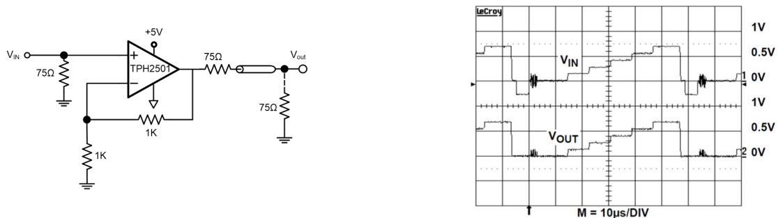
Figure 18. Sync Pulse Remover and Waveform
