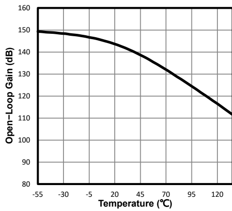
Figure 13. Open-Loop Gain vs. Temperature
