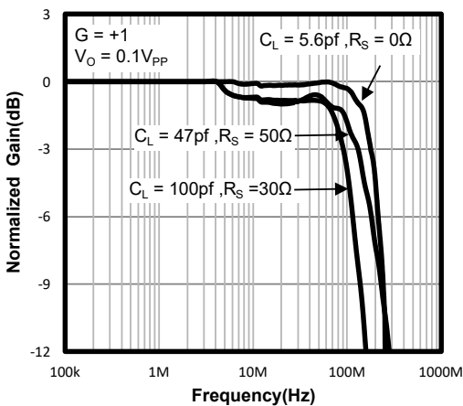
Figure 9. Frequency Response vs. Capacitive Load
