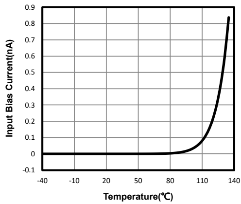
Figure 15. Input Bias Current vs. Temperature
