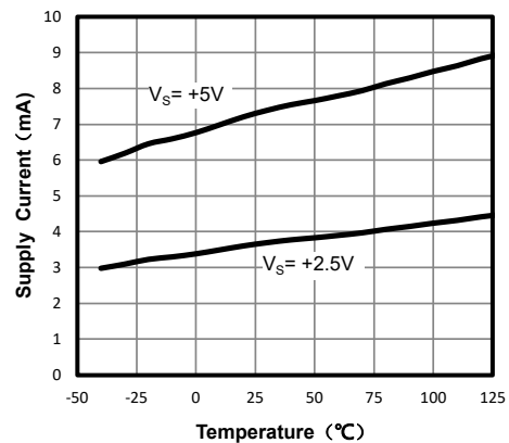
Figure 6. Quiescent Current vs. Temperature
