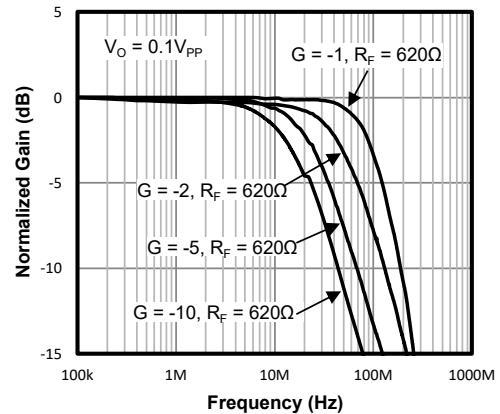
Figure 2. Inverting Small-Signal Frequency Response
