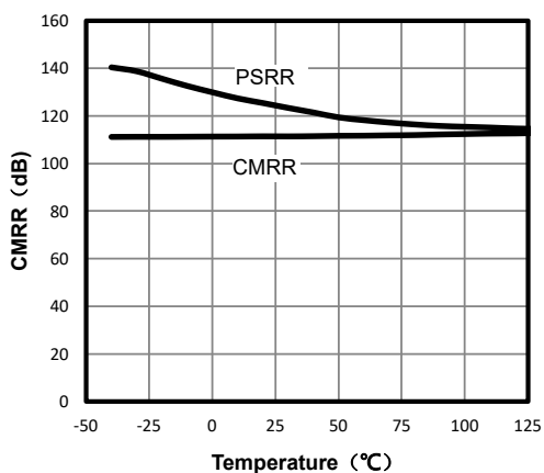
Figure 7. CMRR and PSRR vs. Temperature
