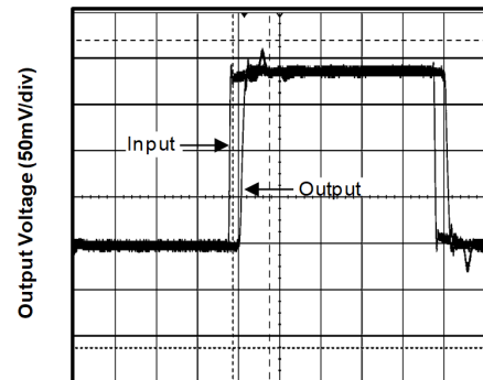
Figure 4. Non-Inverting Small-Signal Step Response
