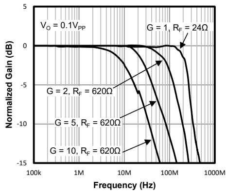
Figure 1. Non-Inverting Small-Signal Frequency Response
