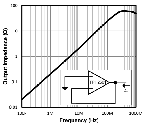
Figure 11. Closed-Loop Output Impedance vs. Frequency
