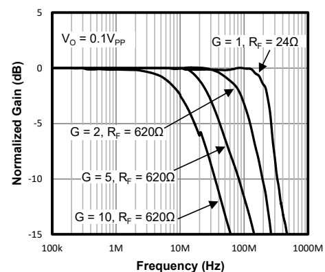
Non-Inverting Small-Signal Frequency Response
