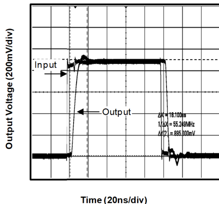
Figure 5. Inverting Large-Signal Step Response
