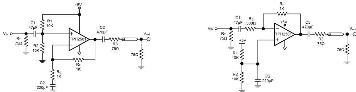
Figure 17. 5-V Single-Supply Non-Inverting and Inverting Video-Line Driver
