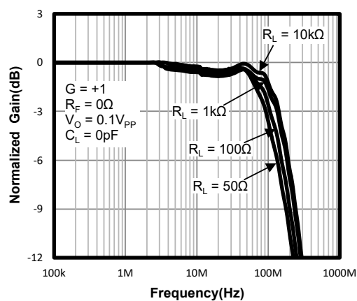
Figure 8. Frequency Response for Various R_L
