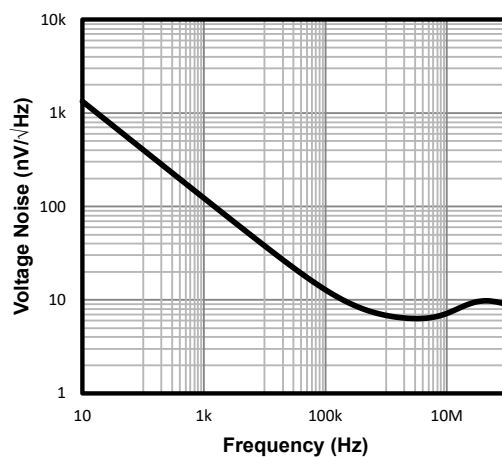
Figure 12. Voltage Spectral Density vs. Frequency
