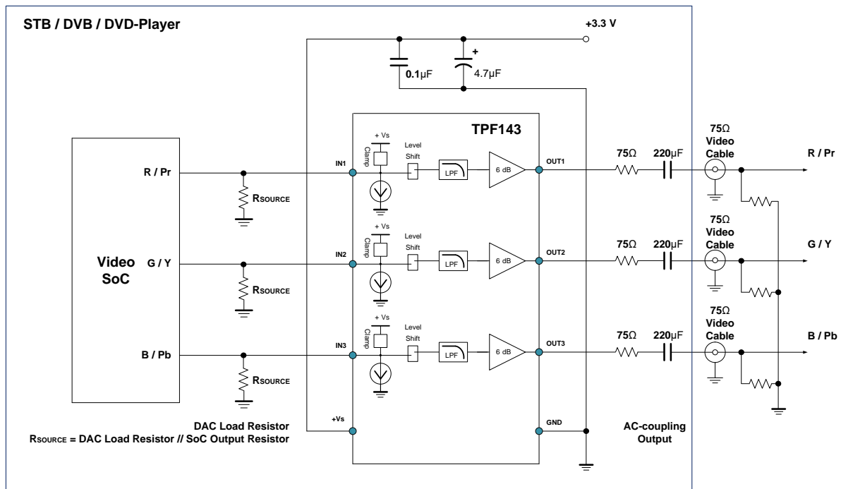
Figure13. Reference Design
