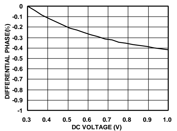
Figure12. Differential Phase(dP)
