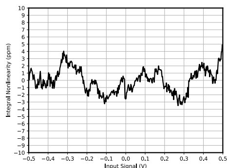
Figure 5. INL vs. Input Signal
