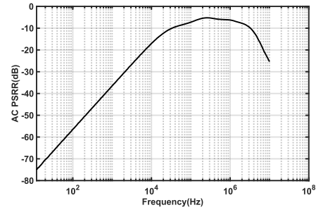
Figure 6. AC PSRR
