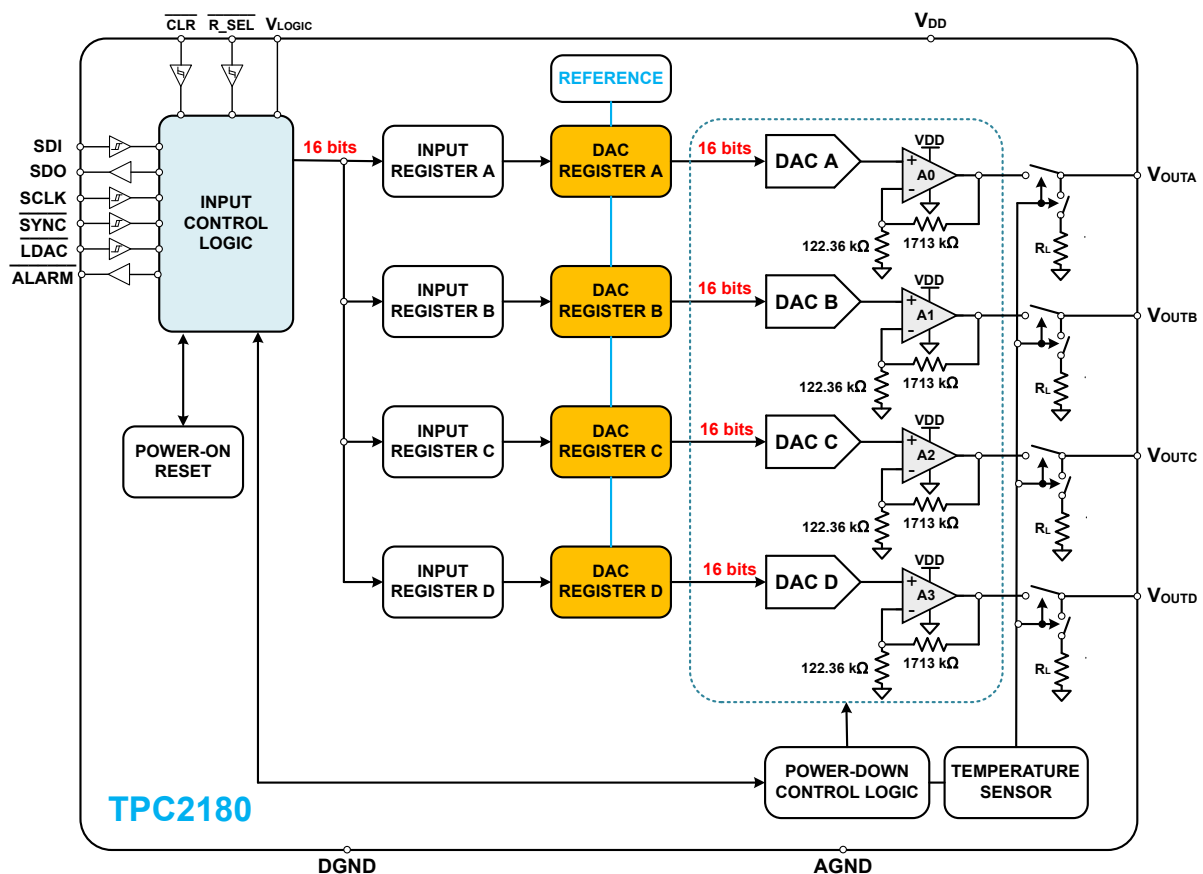
Figure 15. Functional Block Diagram
