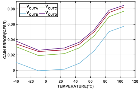
Figure 5. Gain Error vs. Temperature
