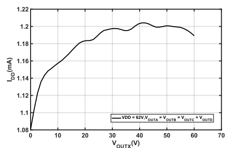
Figure 14. I_{DD} vs. V_{OUTA} to V_{OUTD}
