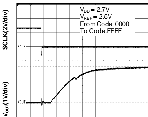
Time (430ns/div)
