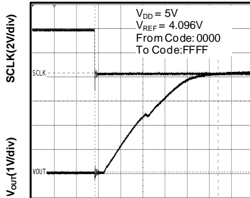
Time (500ns/div)
