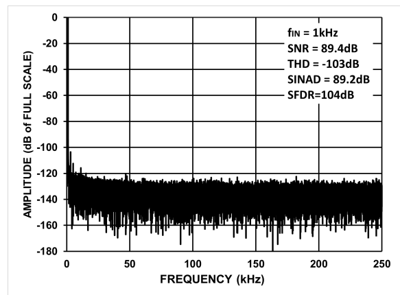
Figure 9. Typical FFT Plot
