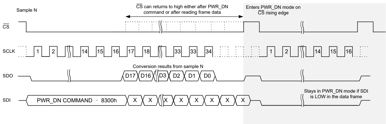
Figure 34. Enter and Remain in PWR_DN Mode Timing Diagram
