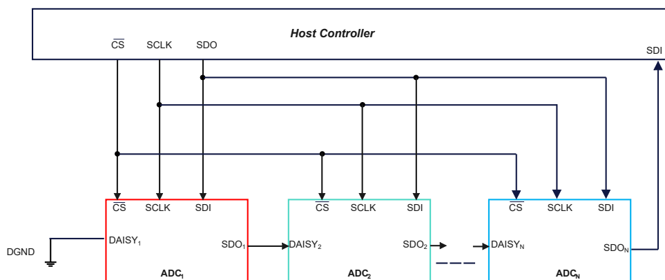
Figure 29. Daisy-Chain Connection Schematic
