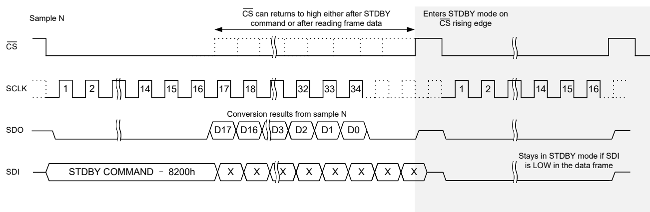
Figure 32. Enter and Remain in STDBY Mode Timing Diagram
