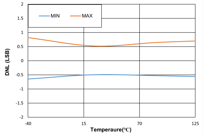
Figure 3. DNL vs. Temperature
