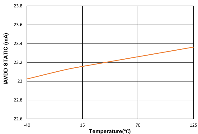
Figure 20. AVDD Current vs. Temperature for the TPAFE51736S8 (Static)
