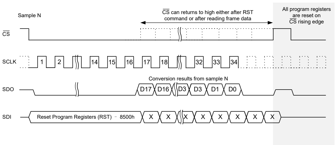
Figure 42. Reset Program Registers (RST) Timing Diagram
