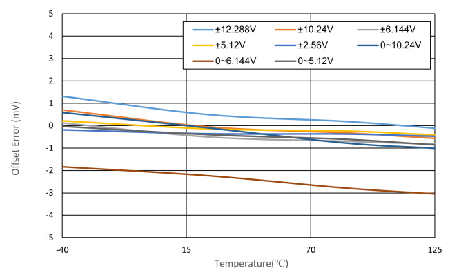
Figure 17. Offset vs. Temperature
