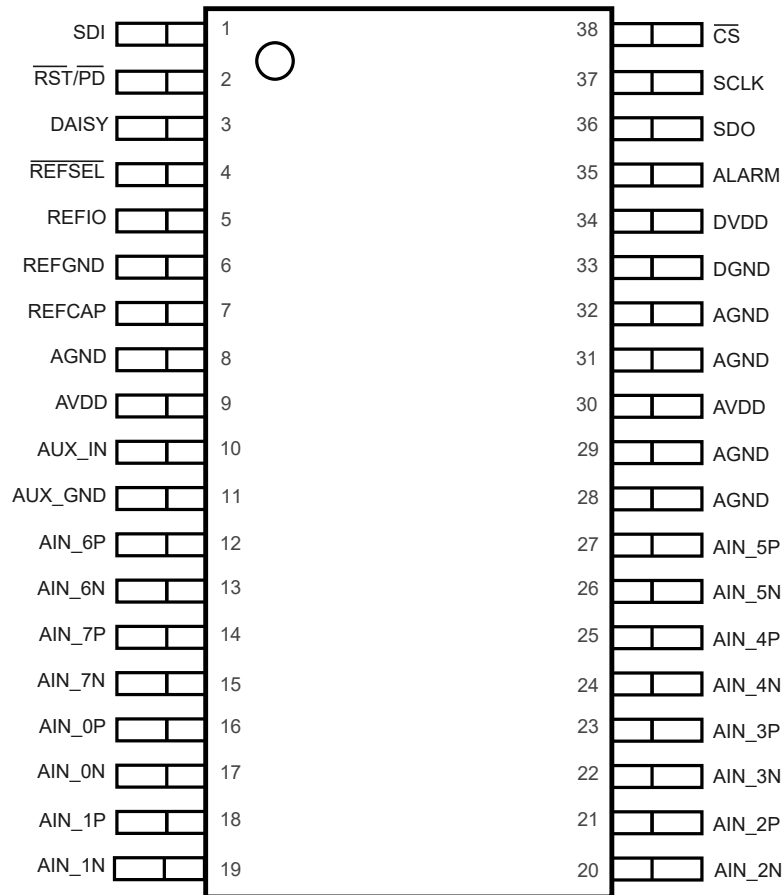
TPAFE51738S8 TSSOP38 Package Top View
