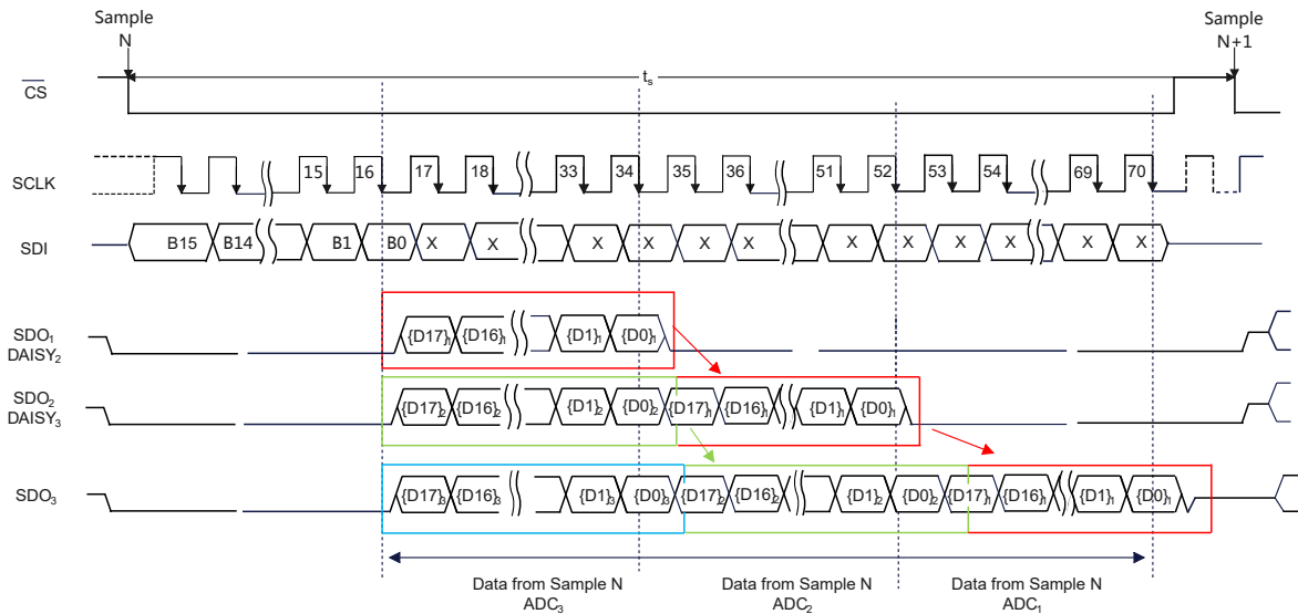
Figure 30. Three Devices Connected in Daisy-Chain Mode Timing Diagram
