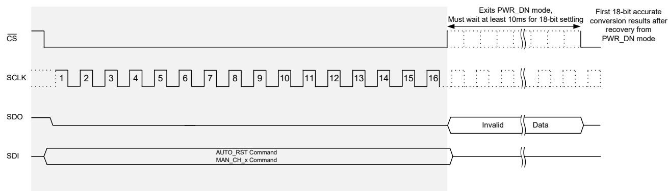
Figure 35. Exit PWR_DN Mode Timing Diagram
