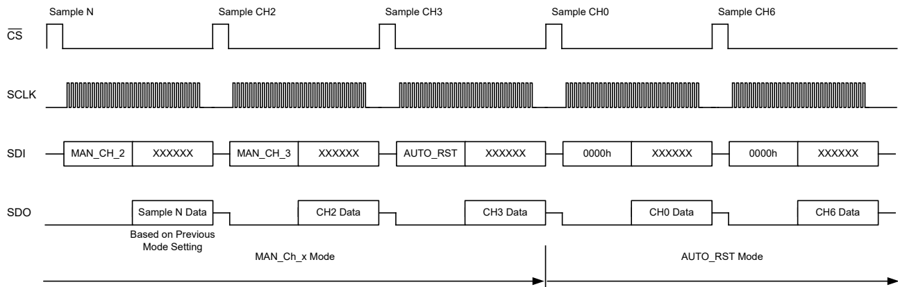
Figure 41. Transitioning from MAN_Ch_n to AUTO_RST Mode (Channels 0 and 6 are Selected for Auto Sequence)
