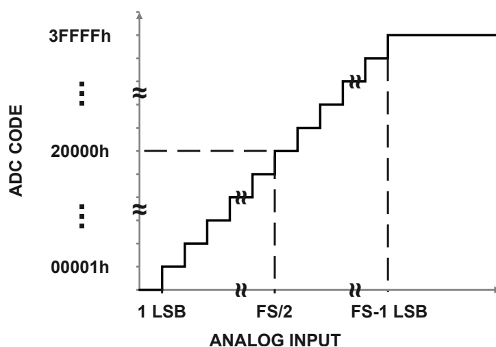
Figure 25. 18-Bit ADC Transfer Function (Straight-Binary Format)
