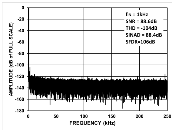
Figure 8. Typical FFT Plot
