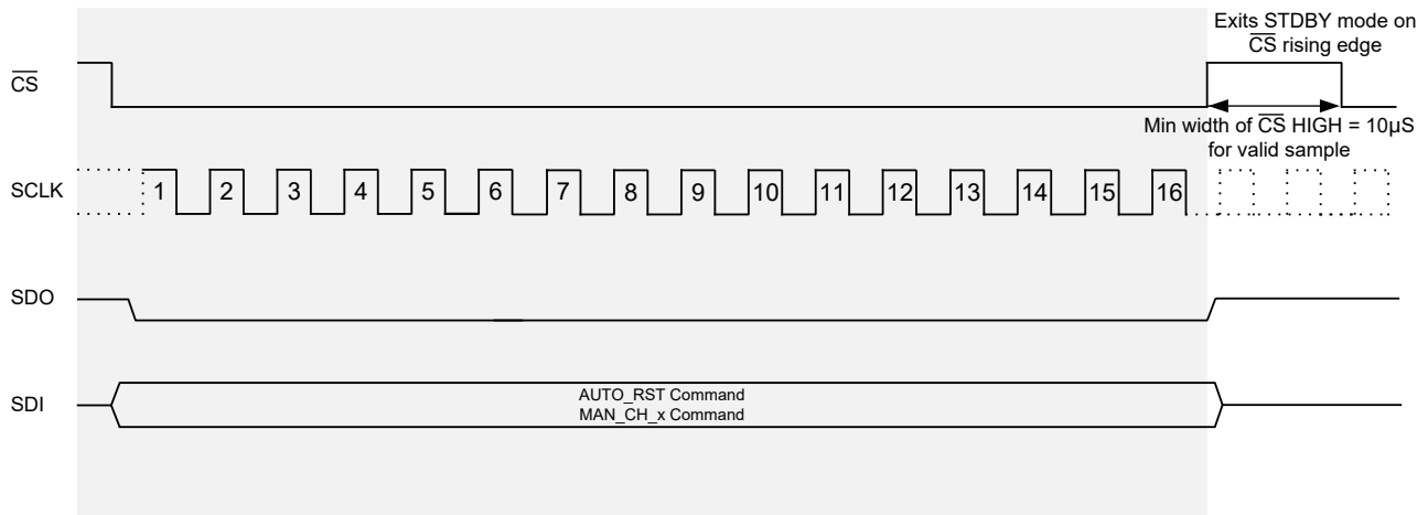
Figure 33. Exit STDBY Mode Timing Diagram
