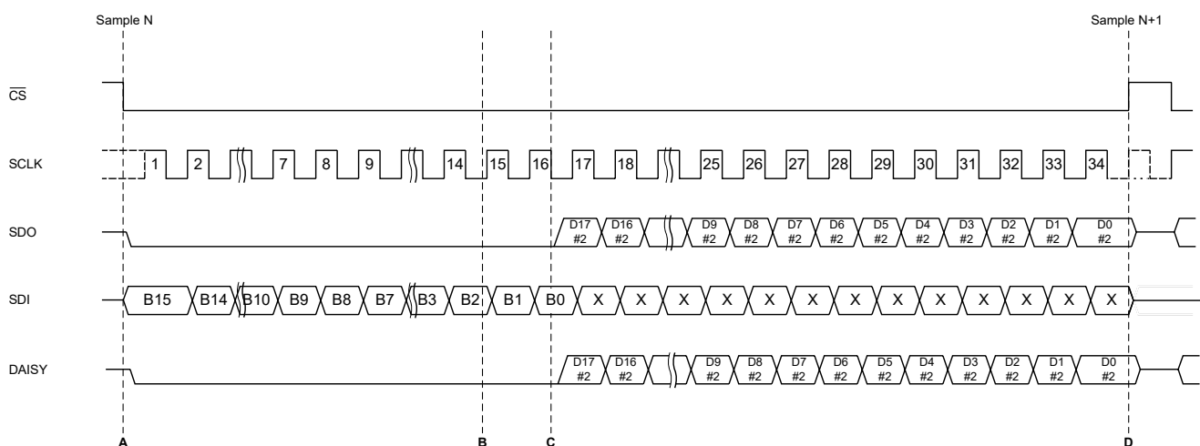
Figure 28. Device Operation Using the Serial Interface Timing Diagram
