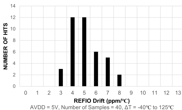
Figure 19. Internal Reference Temperature Drift Histogram
