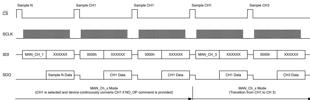
Figure 39. Device Operation in MAN_Ch_n Mode
