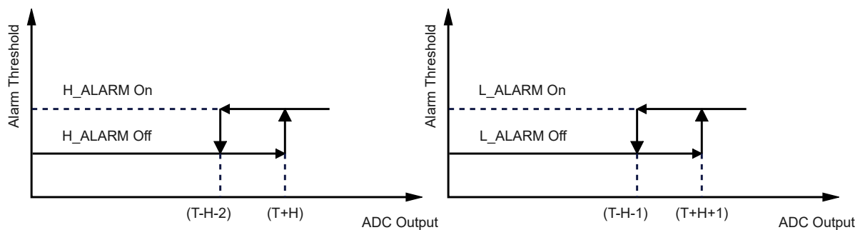
Figure 26. High-ALARM and Low-ALARM Hysteresis
