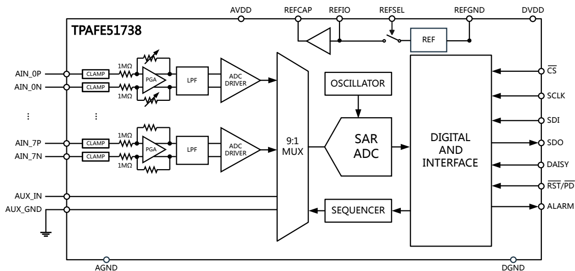
Figure 22. TPAFE51738S8 Block Diagram
