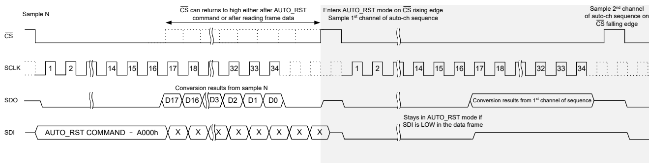
Figure 36. Enter AUTO_RST Mode Timing Diagram
