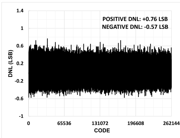
Figure 2. Typical DNL for All Codes
