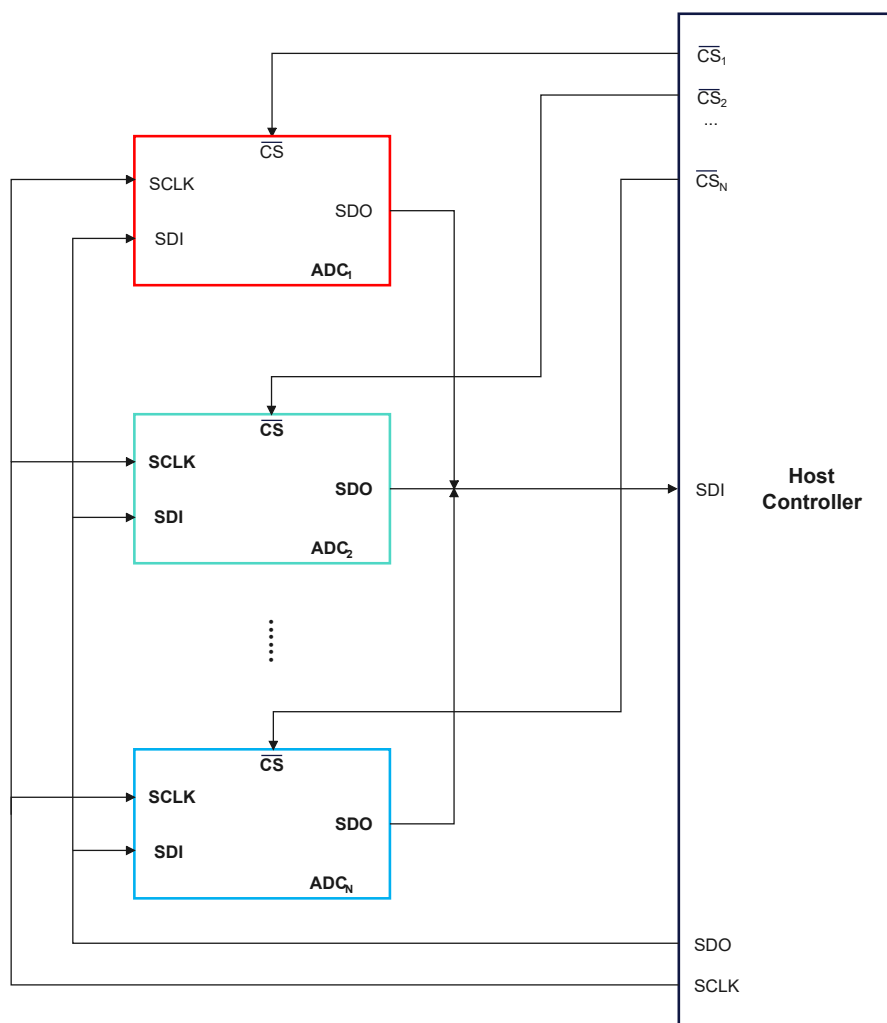
Figure 31. Star Connection Schematic
