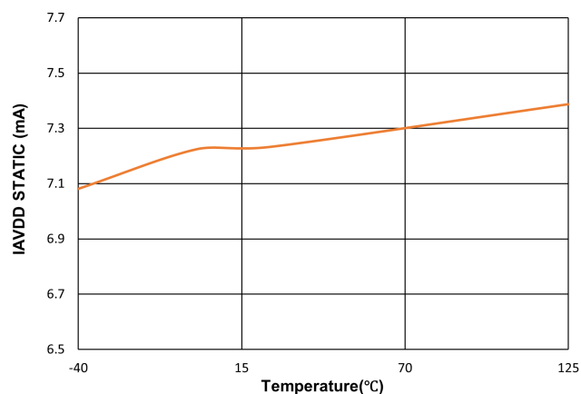
Figure 21. AVDD Current vs. Temperature for the TPAFE51736S8 (STANDBY)
