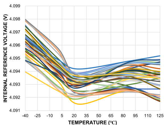
Figure 18. Internal Reference vs. Temperature
