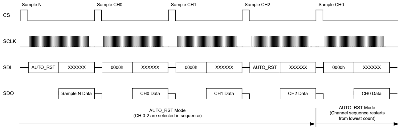
Figure 37. Device Operation Example in AUTO_RST Mode
