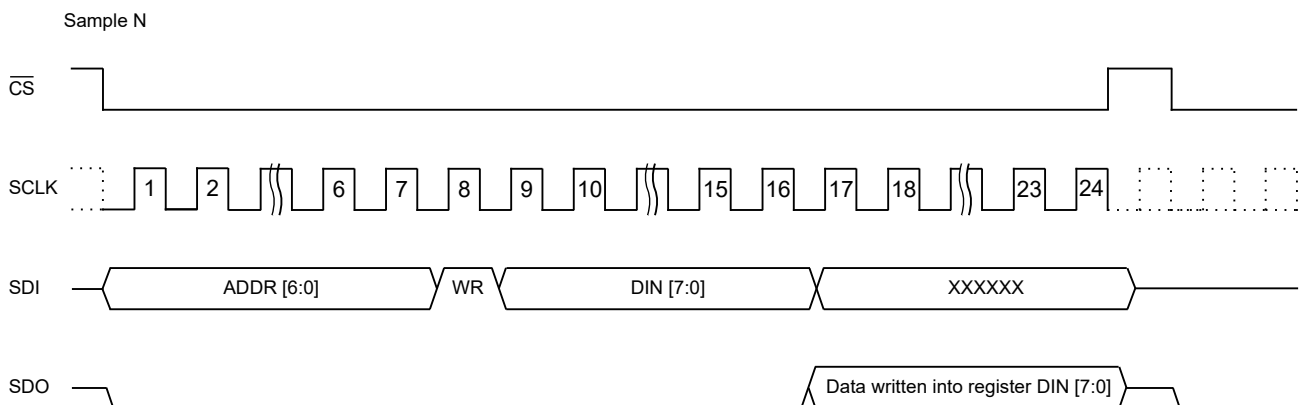
Figure 43. Program Register Write Cycle Timing Diagram
