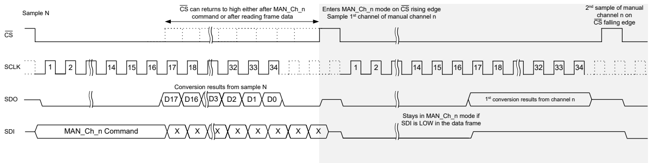
Figure 38. Enter MAN_Ch_n Scan Mode Timing Diagram
