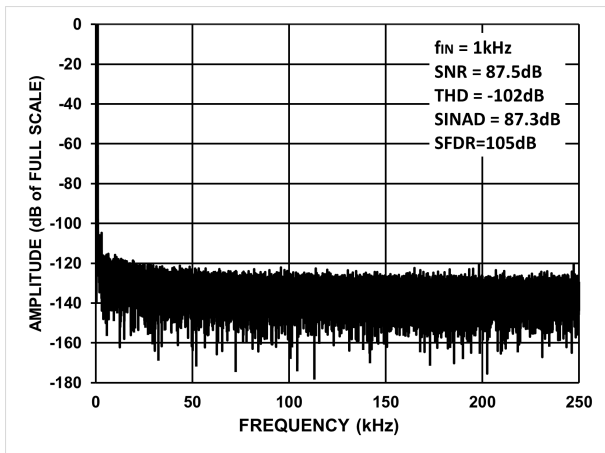
Figure 12. Typical FFT Plot
