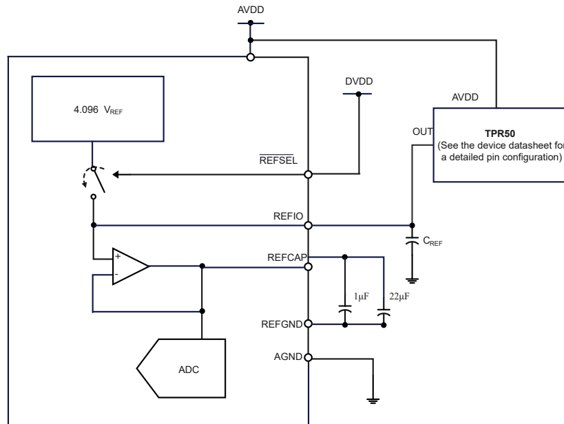
Figure 24. Device Connections for Using an External 4.096-V Reference
