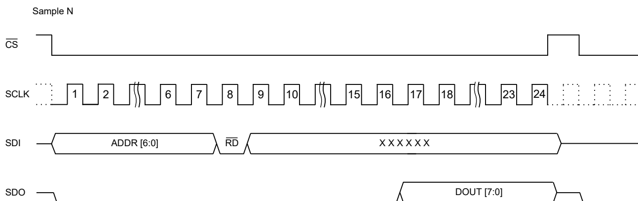
Figure 44. Program Register Read Cycle Timing Diagram
