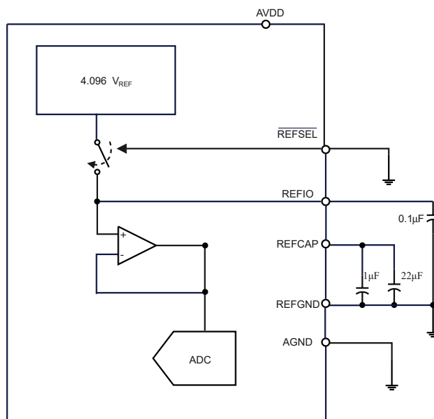
Figure 23. Device Connections for Using an Internal 4.096-V Reference
