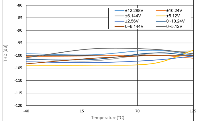
Figure 15. THD vs. Temperature
