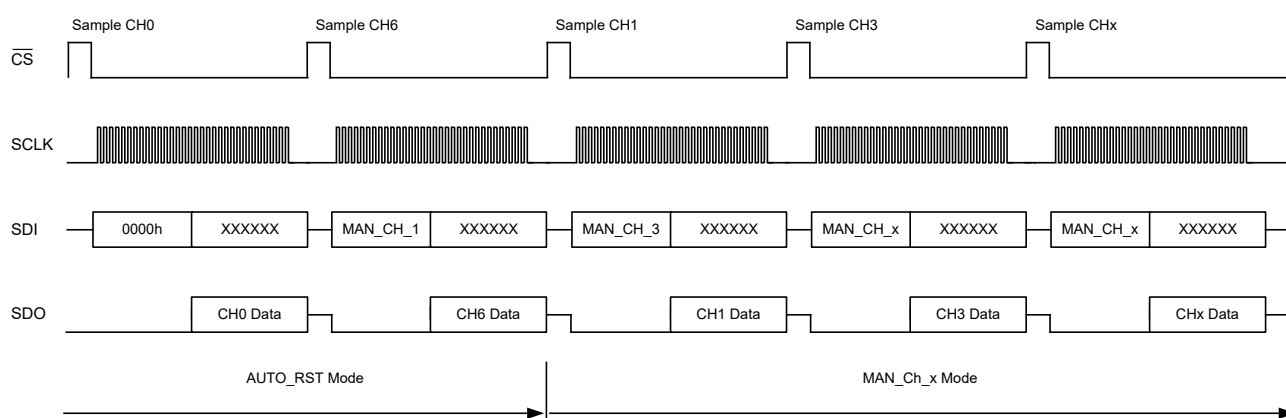
Figure 40. Transitioning from AUTO_RST to MAN_Ch_n Mode (Channels 0 and 6 are Selected for Auto Sequence)
