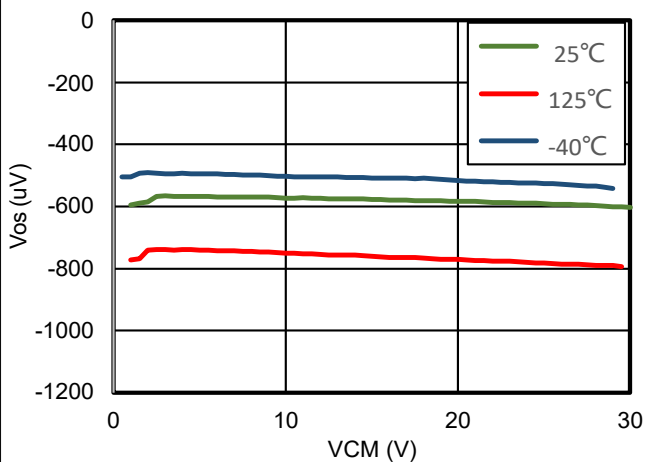
Figure 3. V_{OS} vs. Common-Mode Voltage
