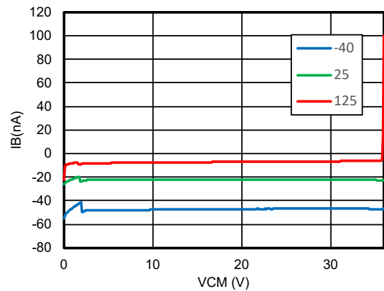
Figure 2. I_B vs. Common-Mode Voltage
