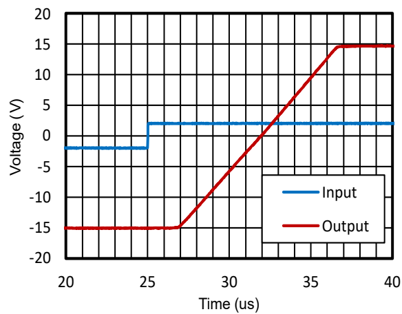
Figure 17. Overload Recovery
