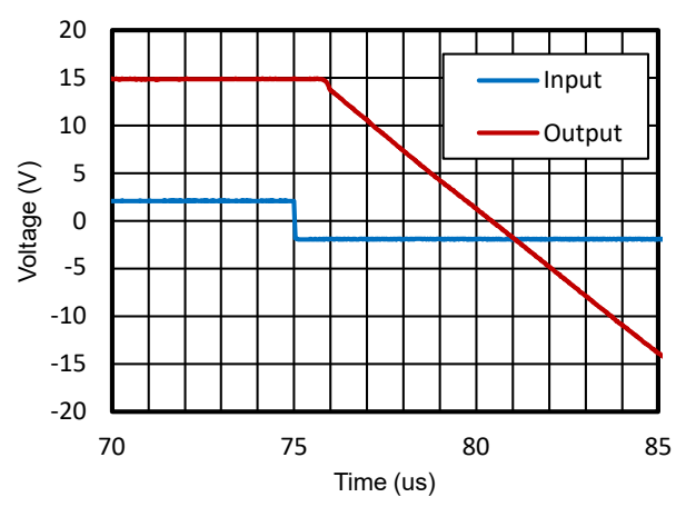
Figure 18. Overload Recovery
