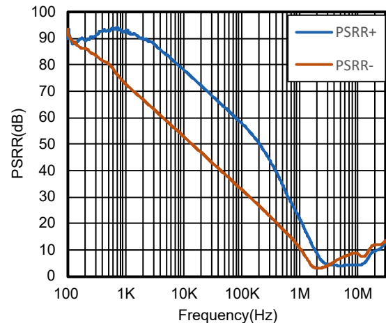
Figure 4. PSRR vs. Frequency
