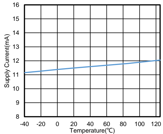
Figure 6. I_q vs. Temperature, +15 V Supply, TPA2682
