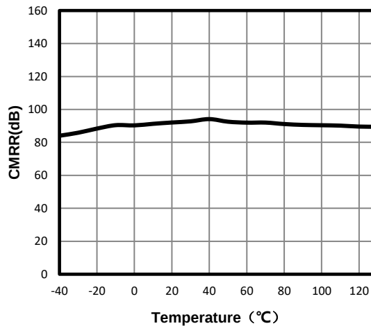
CMRR vs. Temperature
