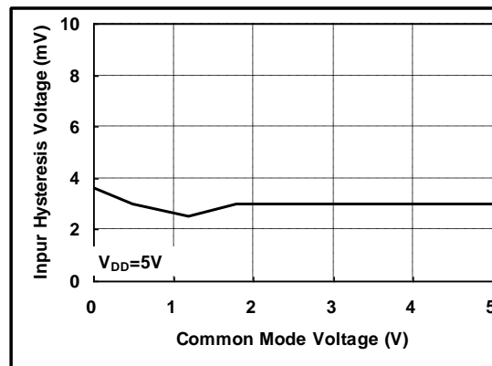
Input Hysteresis Voltage vs. Common Mode Voltage
