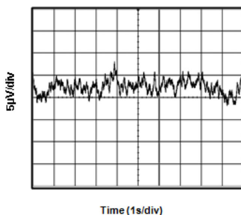
Figure 12. 0.1-Hz to 10-Hz Input Voltage Noise
