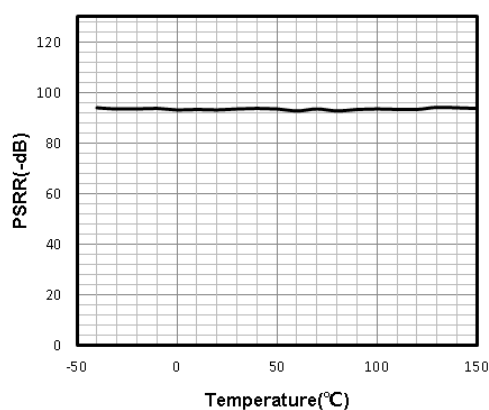
Figure 10. PSRR vs. Temperature
