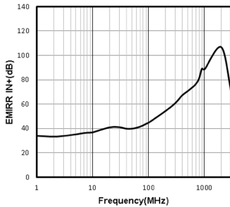
Figure 13. EMIRR IN+ vs. Frequency
