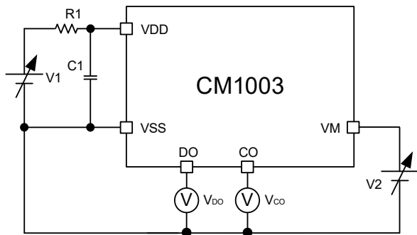
Figure 6 Test Circuits 1
