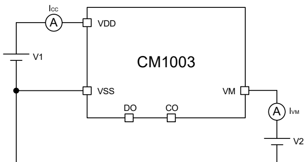
Figure 8 Test Circuits 3
