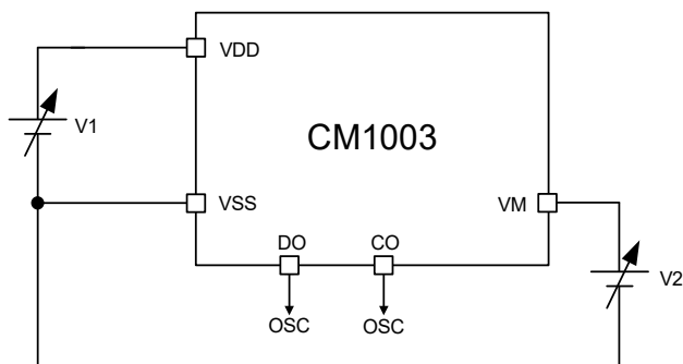
Figure 10 Test Circuits 5
