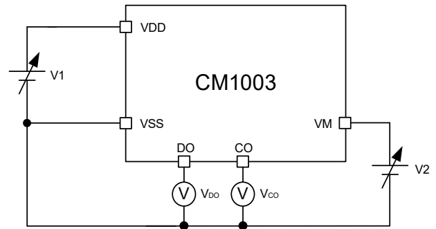
Figure 7 Test Circuits 2
