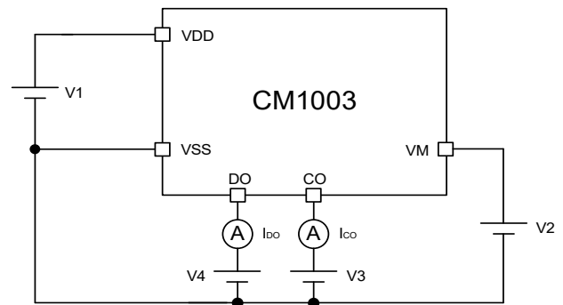
Figure 9 Test Circuits 4
