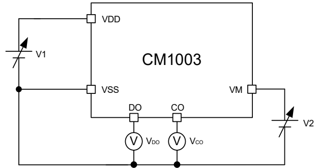
Figure 10 Test Circuits 2
