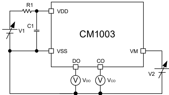
Figure 9 Test Circuits 1
