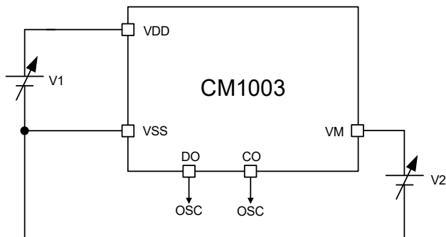
Figure 13 Test Circuits 5
