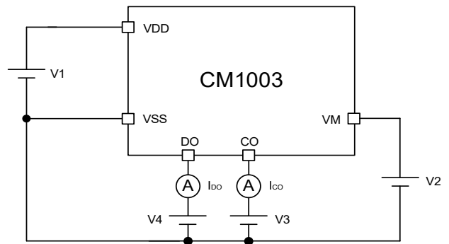
Figure 12 Test Circuits 4
