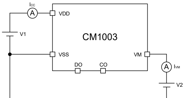
Figure 11 Test Circuits 3
