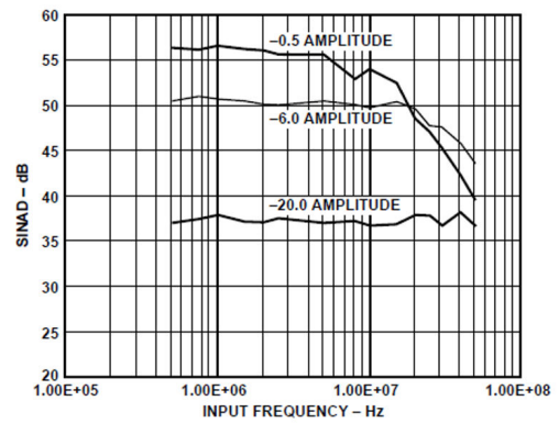
Figure 2. SINAD vs. Input Frequency
