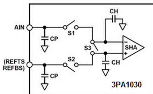
Figure 17. 3PA1030 Equivalent Input Structure
