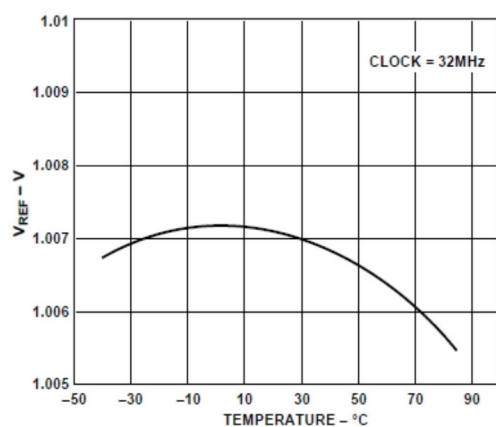
Figure 7. Voltage Reference Error vs. Temperature
