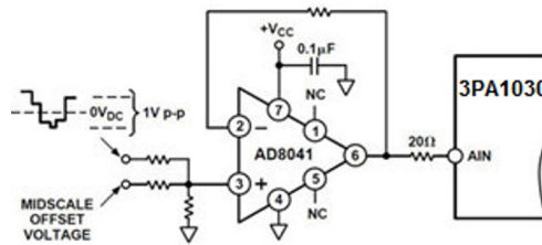
Figure 20. Bipolar Level Shift
