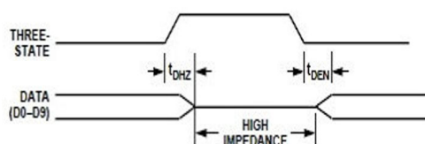
Figure 24. Three-State Timing Diagram
