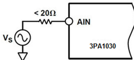
Figure 18. Simple 3PA1030 Drive Configuration
