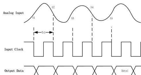
Figure 22. Timing Diagram
