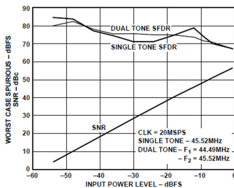
Figure 26. SNR/SFDR for IF @ 45 MHz
