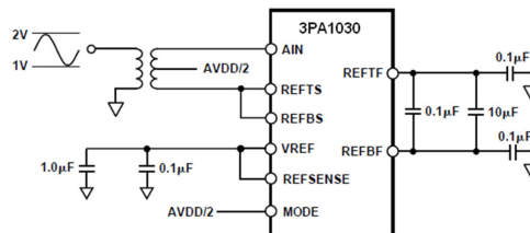
Figure 21. Differential Input
