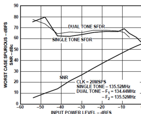
Figure 29. SNR/SFDR for IF @ 135 MHz
