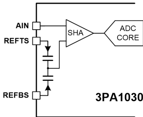
Figure 9. 3PA1030 Equivalent Functional Input Circuit
