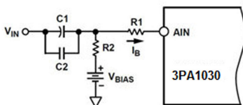
Figure 19. AC Coupled Input
