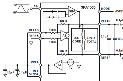
Figure 12. Internal Reference, 1- V_{P-P} Input Span (Top/Bottom Mode)
