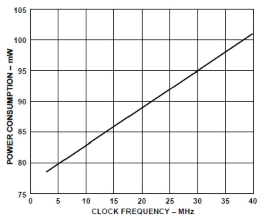
Figure 8. Power Consumption vs. Clock Frequency
