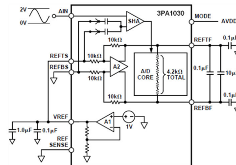
Figure 13. Internal Reference, 2- V_{P-P} Input Span (Top/Bottom Mode)
