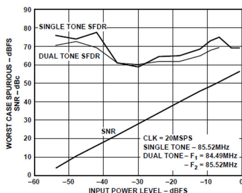
Figure 28. SNR/SFDR for IF @ 85 MHz
