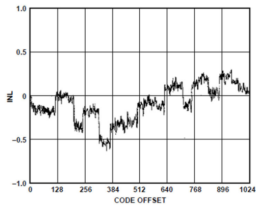
Figure 3. Typical INL
