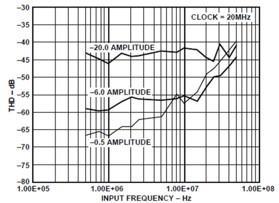
Figure 4. THD vs. Input Frequency
