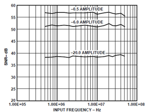
Figure 5. SNR vs. Input Frequency
