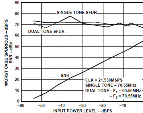
Figure 27. SNR/SFDR for IF @ 70 MHz
