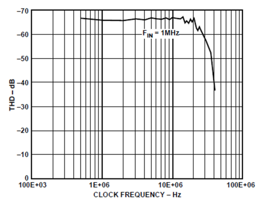
Figure 6. THD vs. Clock Frequency
