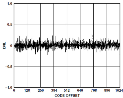
Figure 1. Typical DNL
