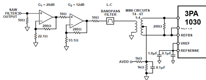
Figure 25. Simplified 3PA1030 IF Sampling Circuit
