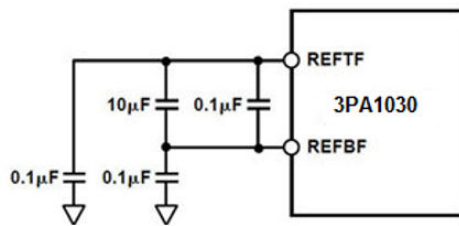
Figure 11. Reference Decoupling Network
